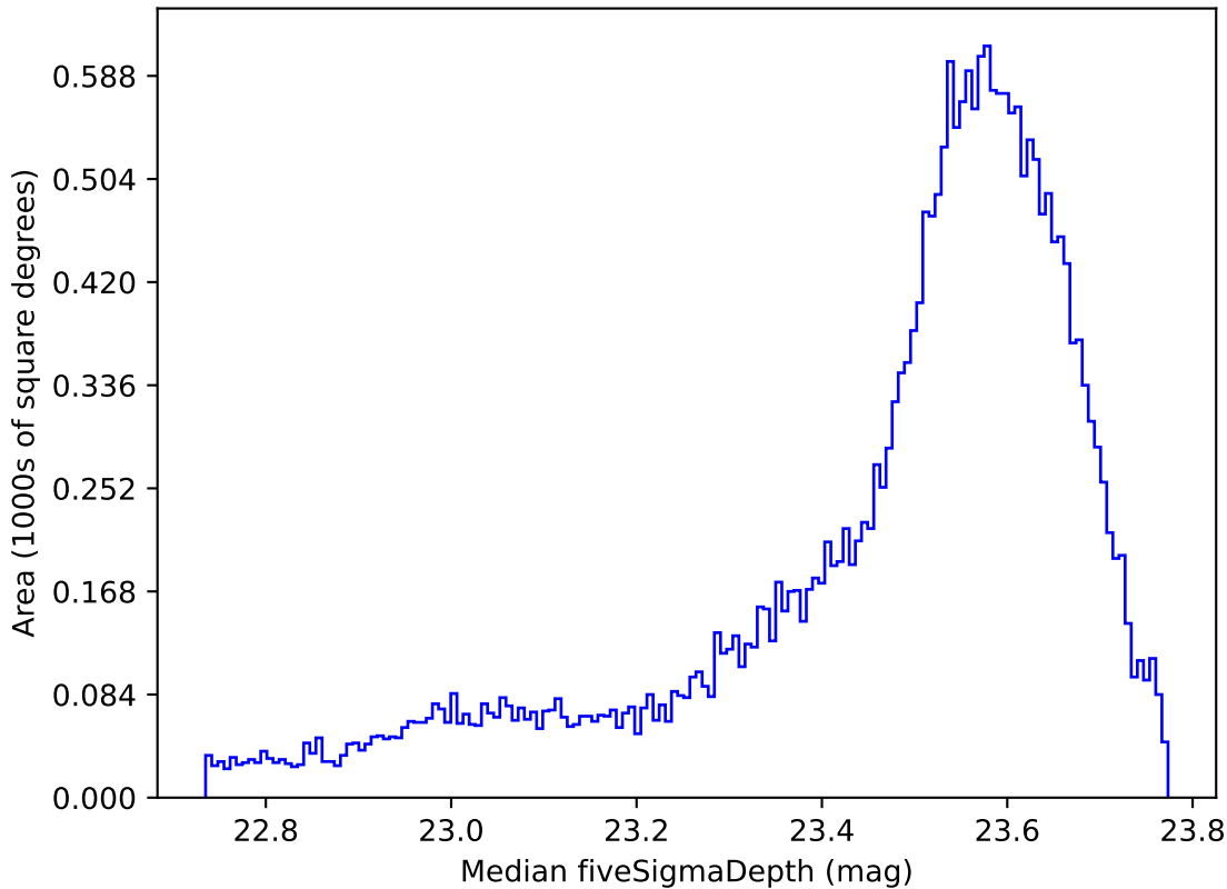
weather_cloudso12v3.4_10yrs All sky i band: Median fiveSigmaDepth
