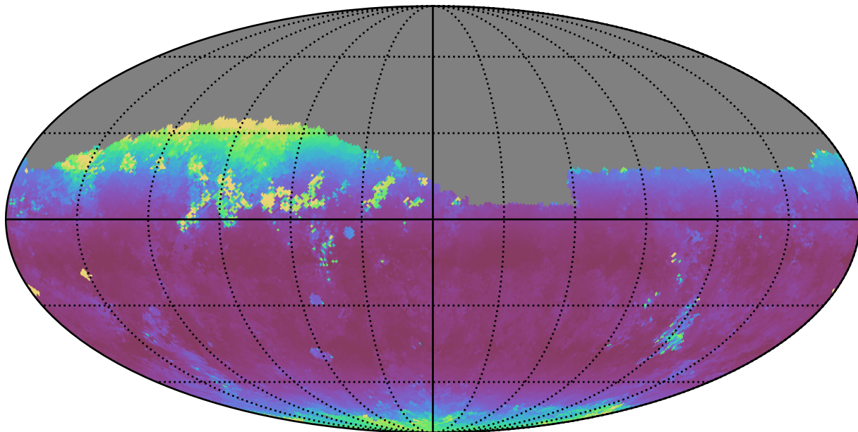
weather_cloudso12v3.4_10yrs Yr 1 z band: Median airmass
