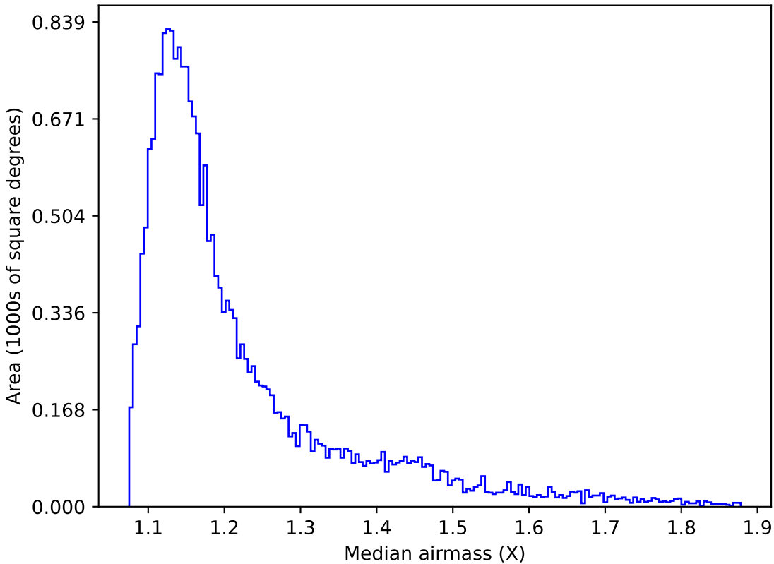
weather_cloudso12v3.4_10yrs Yr 1 y band: Median airmass
