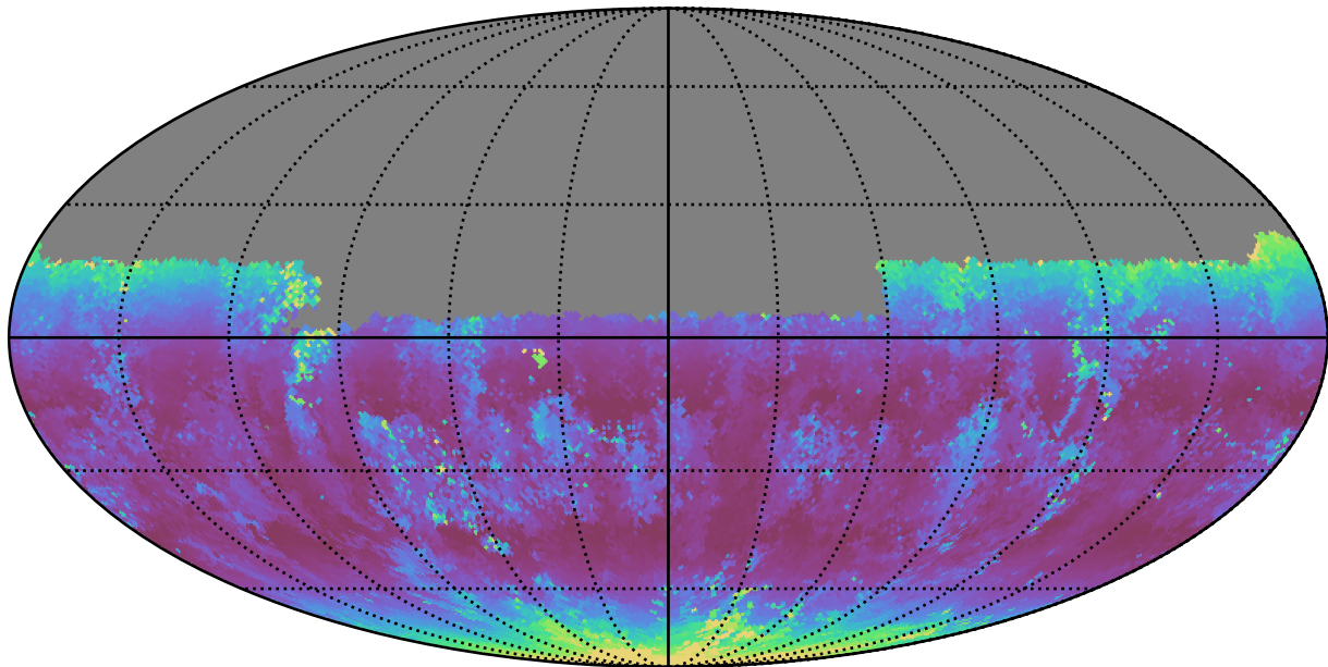
weather_cloudso12v3.4_10yrs Yr 1 u band: Median airmass
