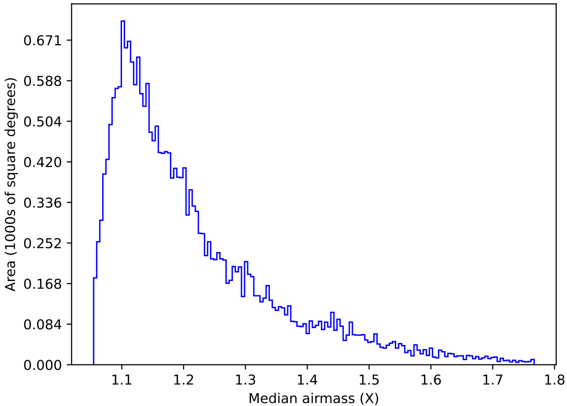
weather_cloudso12v3.4_10yrs Yr 1 u band: Median airmass
