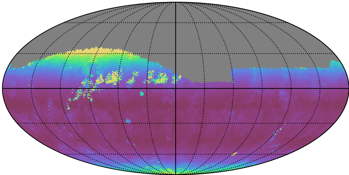
weather_cloudso12v3.4_10yrs Yr 1 r band: Median airmass
