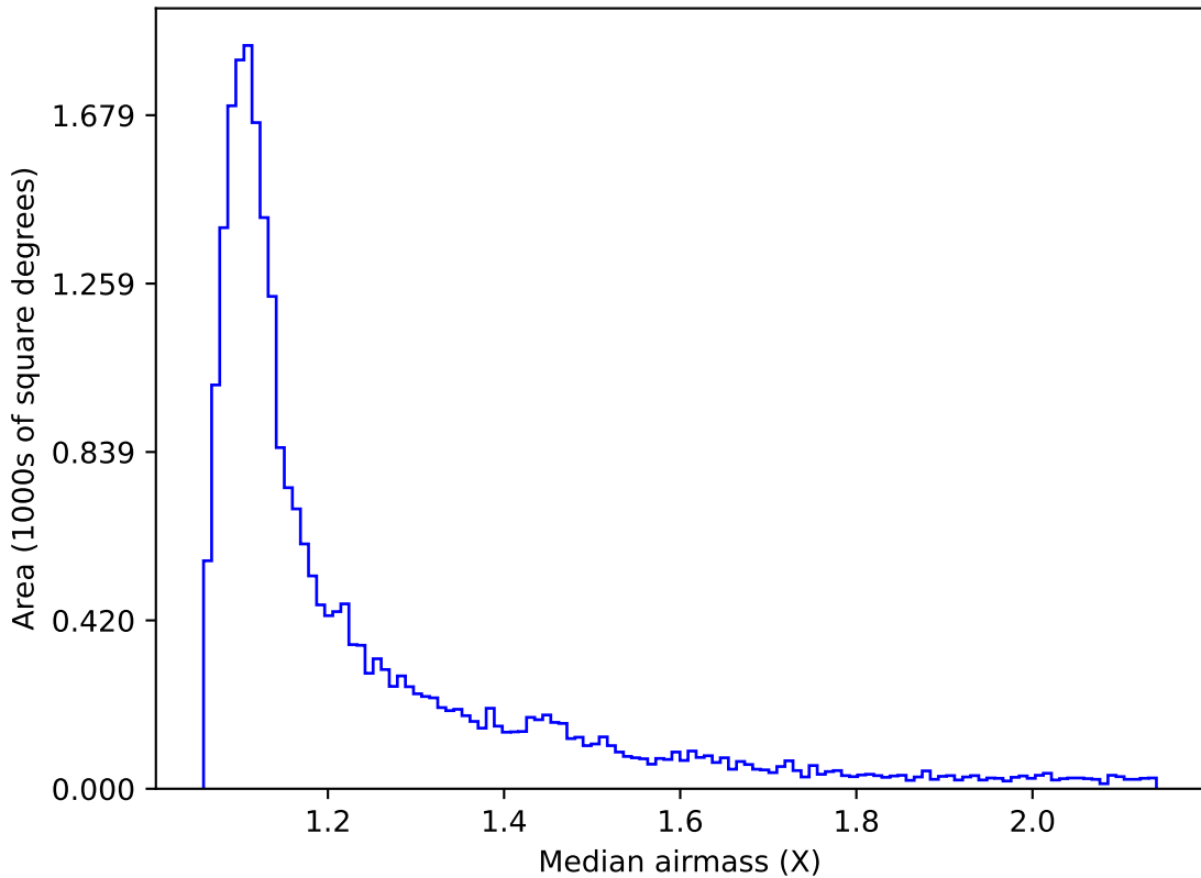
weather_cloudso12v3.4_10yrs Yr 1 r band: Median airmass
