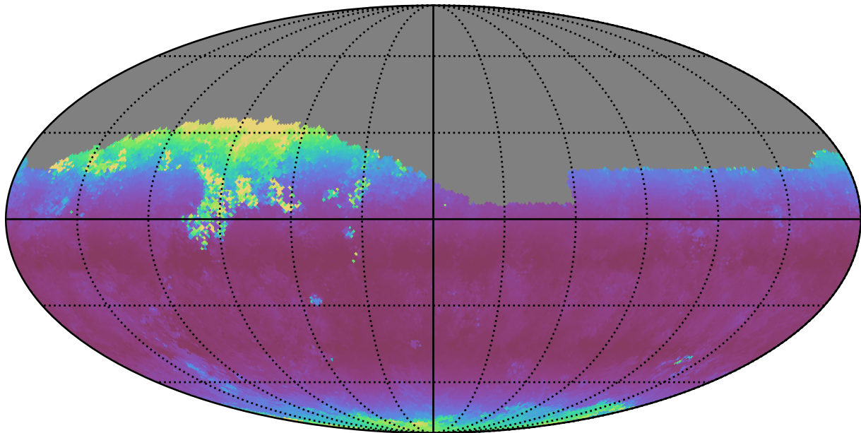
weather_cloudso12v3.4_10yrs Yr 1 i band: Median airmass
