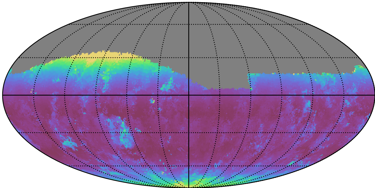
weather_cloudso12v3.4_10yrs Yr 1 g band: Median airmass
