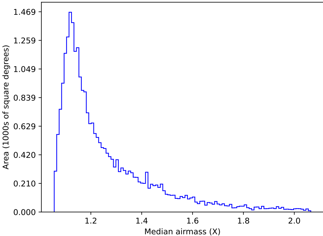
weather_cloudso12v3.4_10yrs Yr 1 g band: Median airmass
