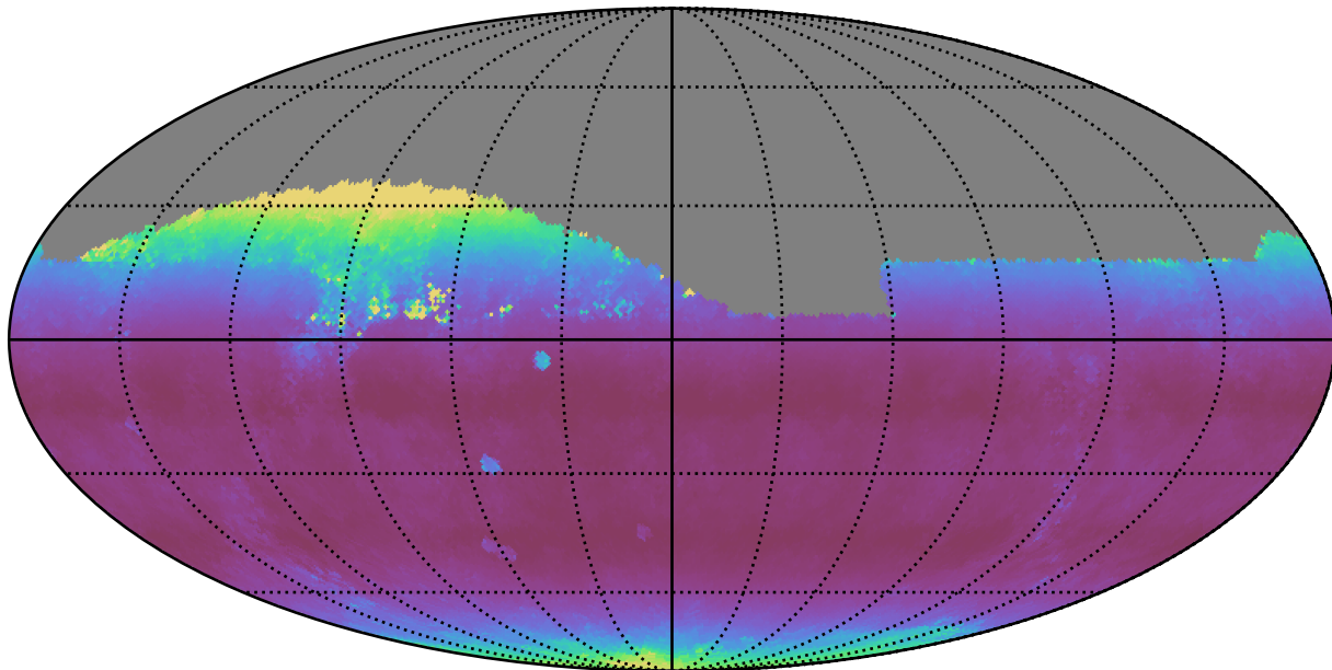
weather_cloudso12v3.4_10yrs Yr 1 all bands: Median airmass
