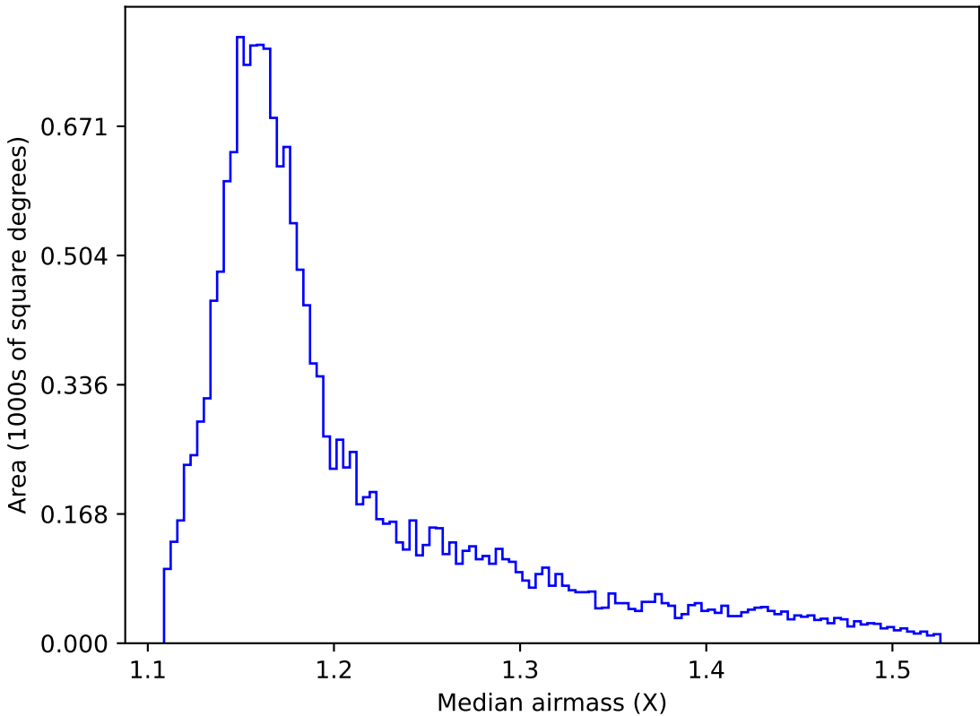
weather_cloudso12v3.4_10yrs WFD y band: Median airmass
