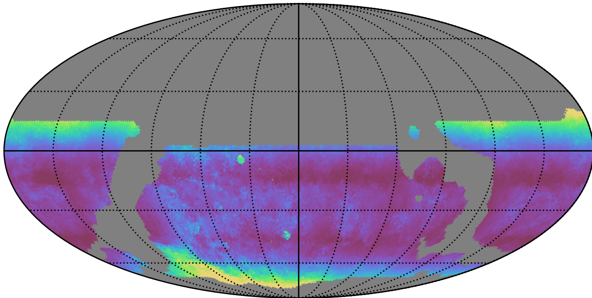
weather_cloudso12v3.4_10yrs WFD u band: Median airmass
