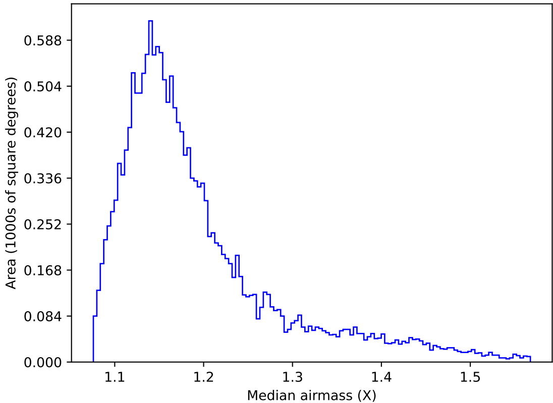
weather_cloudso12v3.4_10yrs WFD u band: Median airmass
