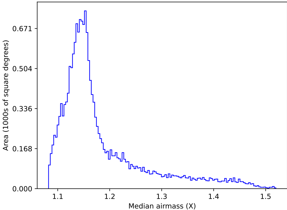
weather_cloudso12v3.4_10yrs WFD r band: Median airmass
