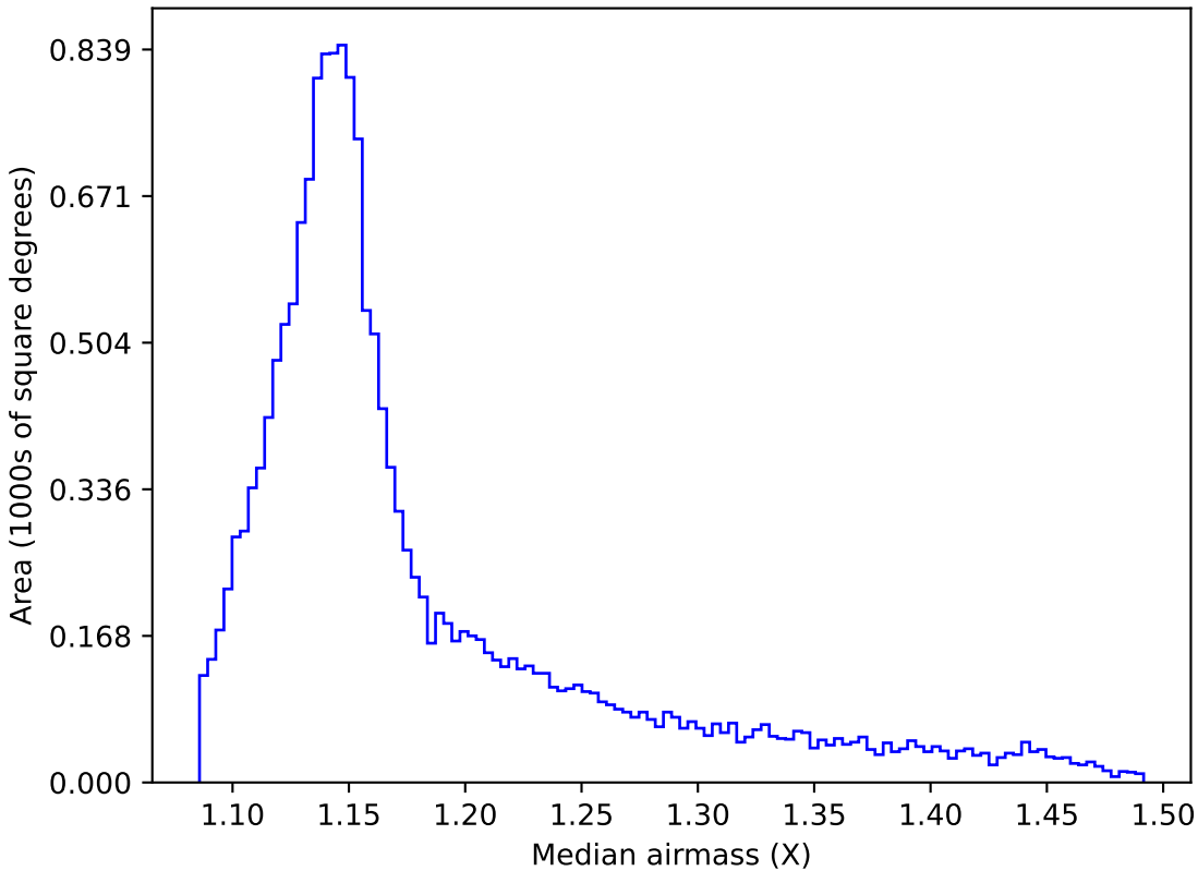
weather_cloudso12v3.4_10yrs WFD i band: Median airmass
