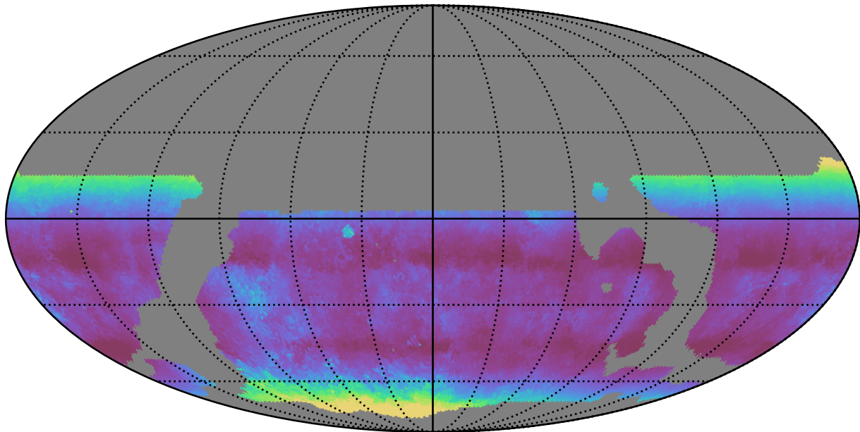
weather_cloudso12v3.4_10yrs WFD g band: Median airmass
