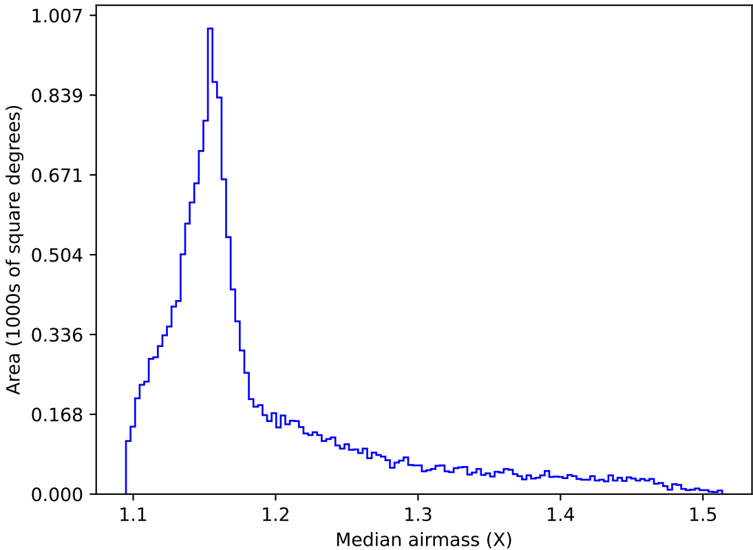
weather_cloudso12v3.4_10yrs WFD all bands: Median airmass
