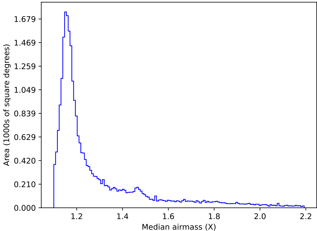
weather_cloudso12v3.4_10yrs All sky z band: Median airmass
