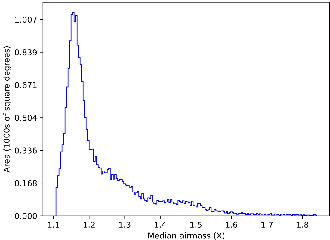
weather_cloudso12v3.4_10yrs All sky y band: Median airmass
