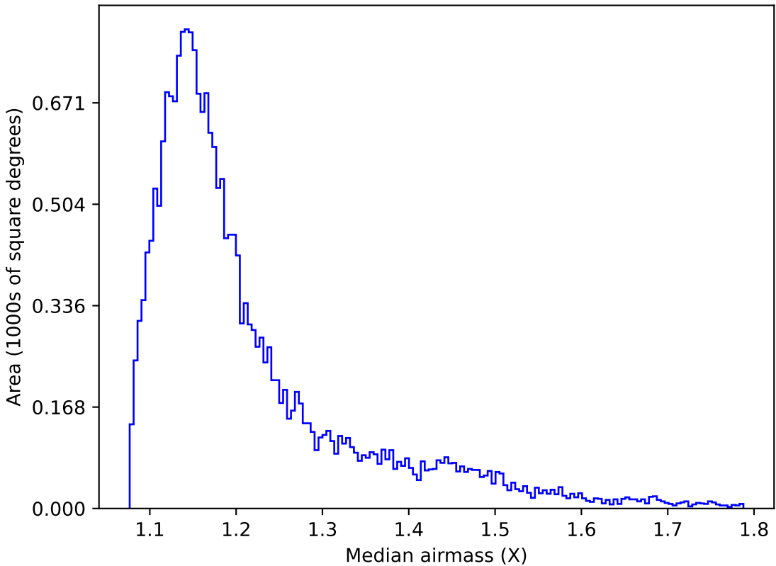
weather_cloudso12v3.4_10yrs All sky u band: Median airmass
