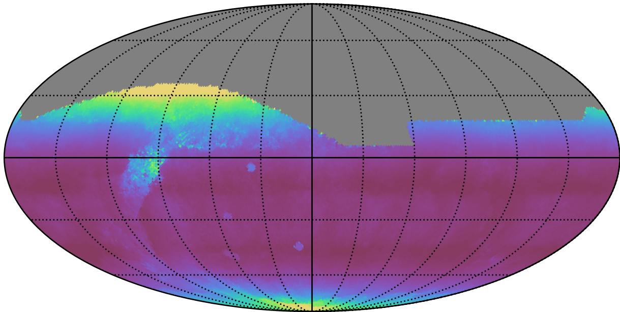
weather_cloudso12v3.4_10yrs All sky r band: Median airmass
