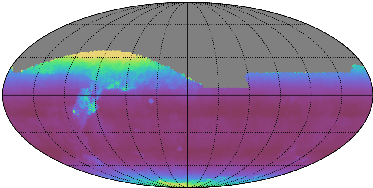
weather_cloudso12v3.4_10yrs All sky i band: Median airmass
