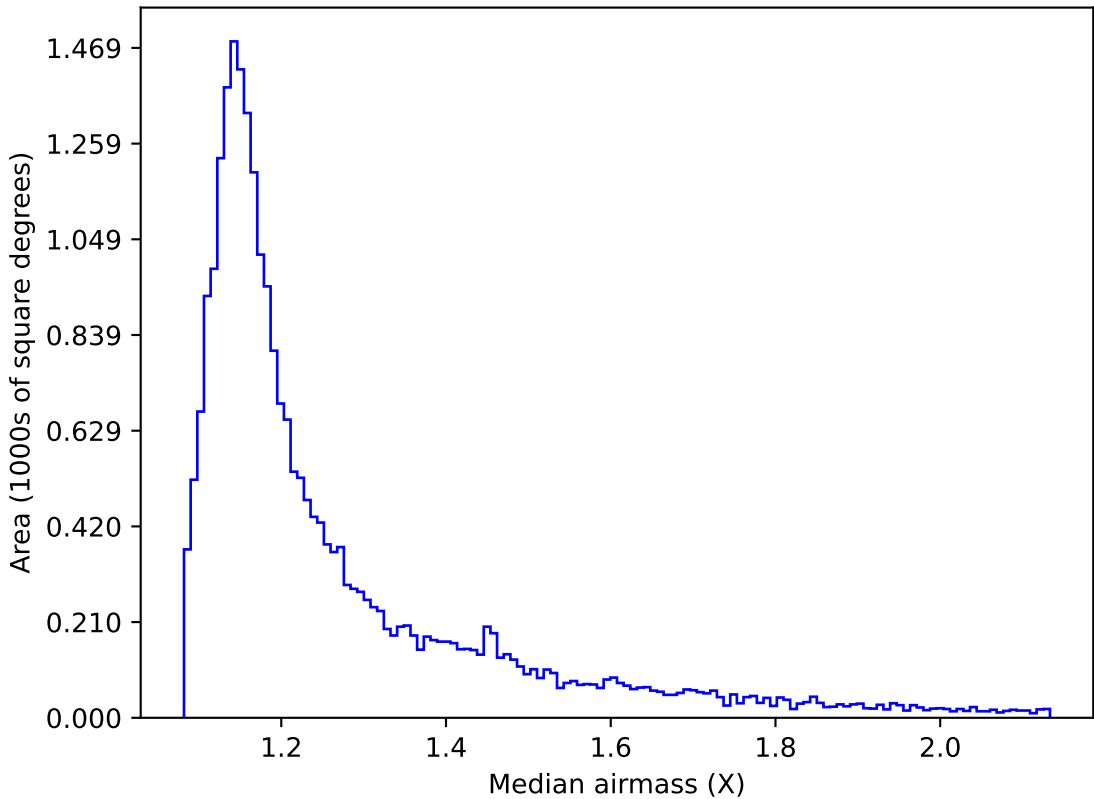
weather_cloudso12v3.4_10yrs All sky g band: Median airmass
