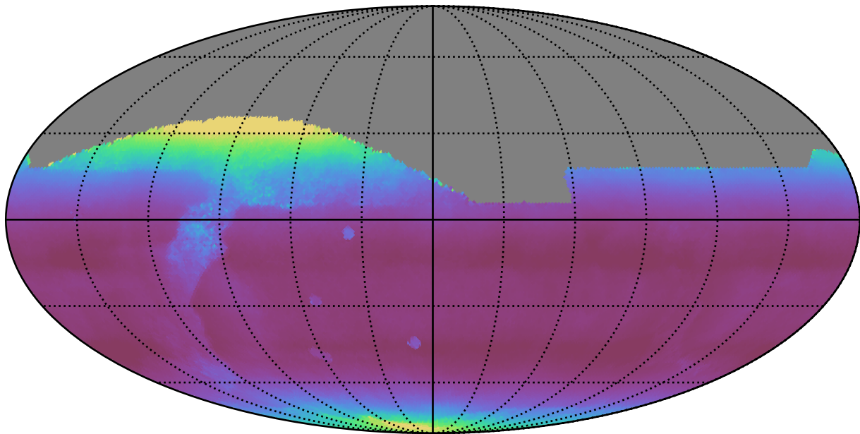
weather_cloudso12v3.4_10yrs All sky all bands: Median airmass
