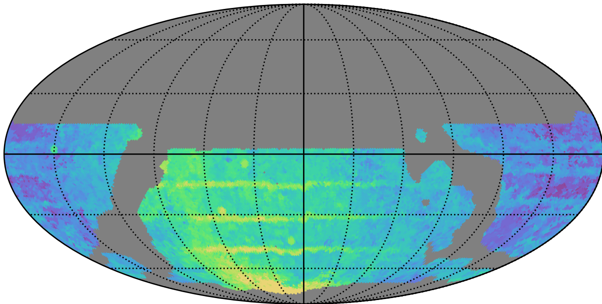
weather_cloudso12v3.4_10yrs WFD z band: Median Season Length
