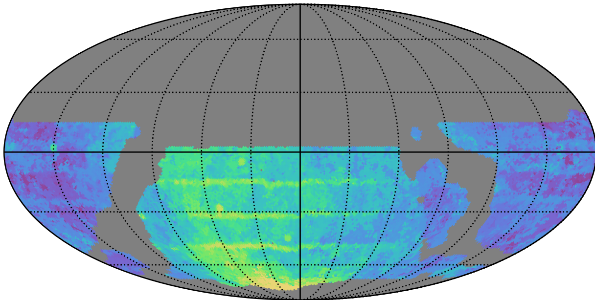
weather_cloudso12v3.4_10yrs WFD y band: Median Season Length
