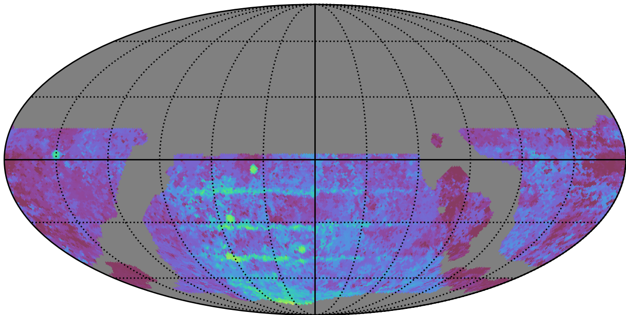
weather_cloudso12v3.4_10yrs WFD u band: Median Season Length
