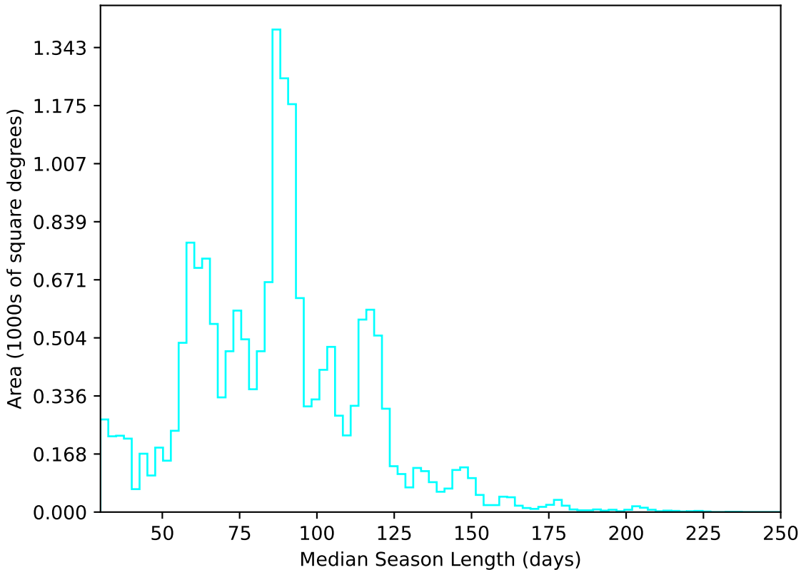
weather_cloudso12v3.4_10yrs WFD u band: Median Season Length
