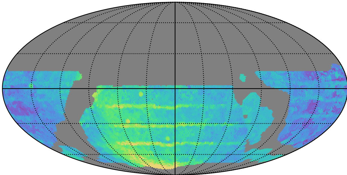
weather_cloudso12v3.4_10yrs WFD r band: Median Season Length
