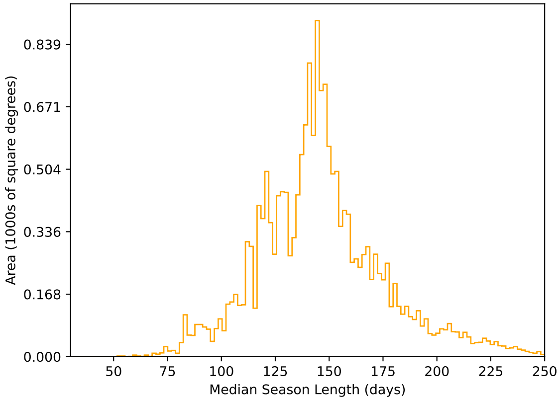
weather_cloudso12v3.4_10yrs WFD r band: Median Season Length
