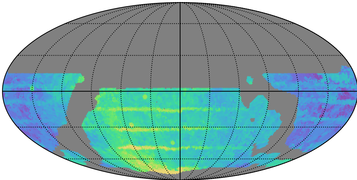
weather_cloudso12v3.4_10yrs WFD i band: Median Season Length
