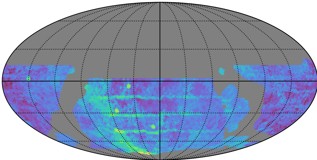
weather_cloudso12v3.4_10yrs WFD g band: Median Season Length
