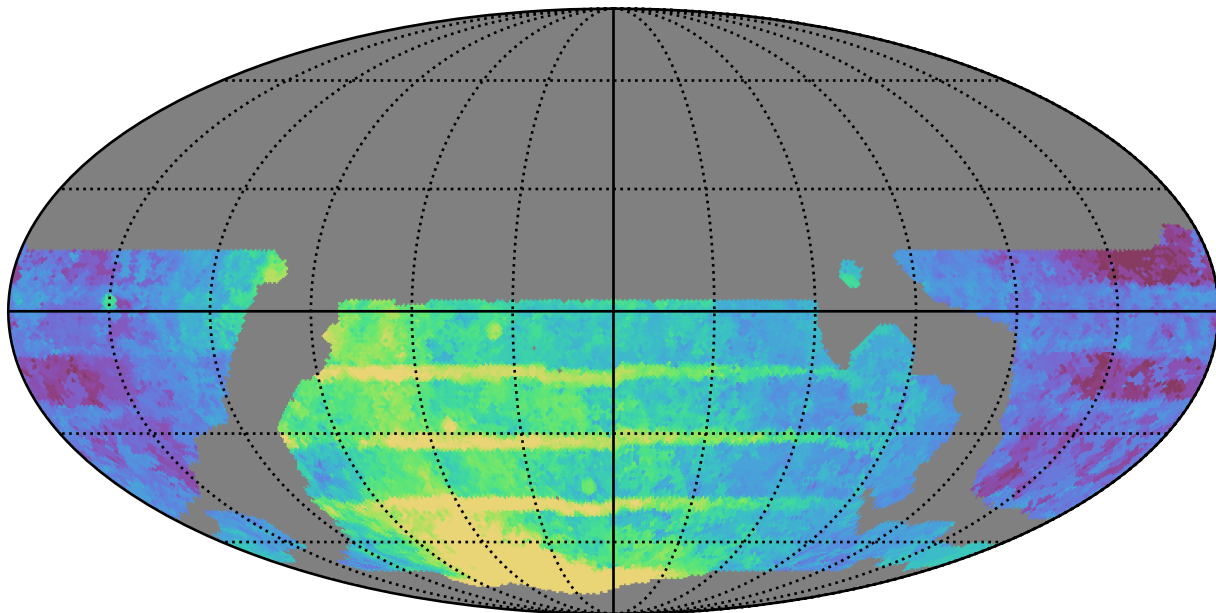
weather_cloudso12v3.4_10yrs WFD all bands: Median Season Length
