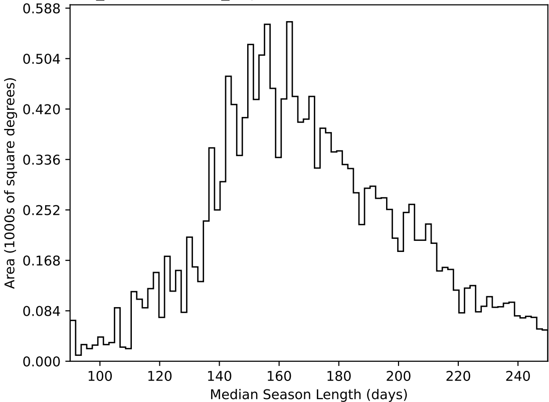
weather_cloudso12v3.4_10yrs WFD all bands: Median Season Length
