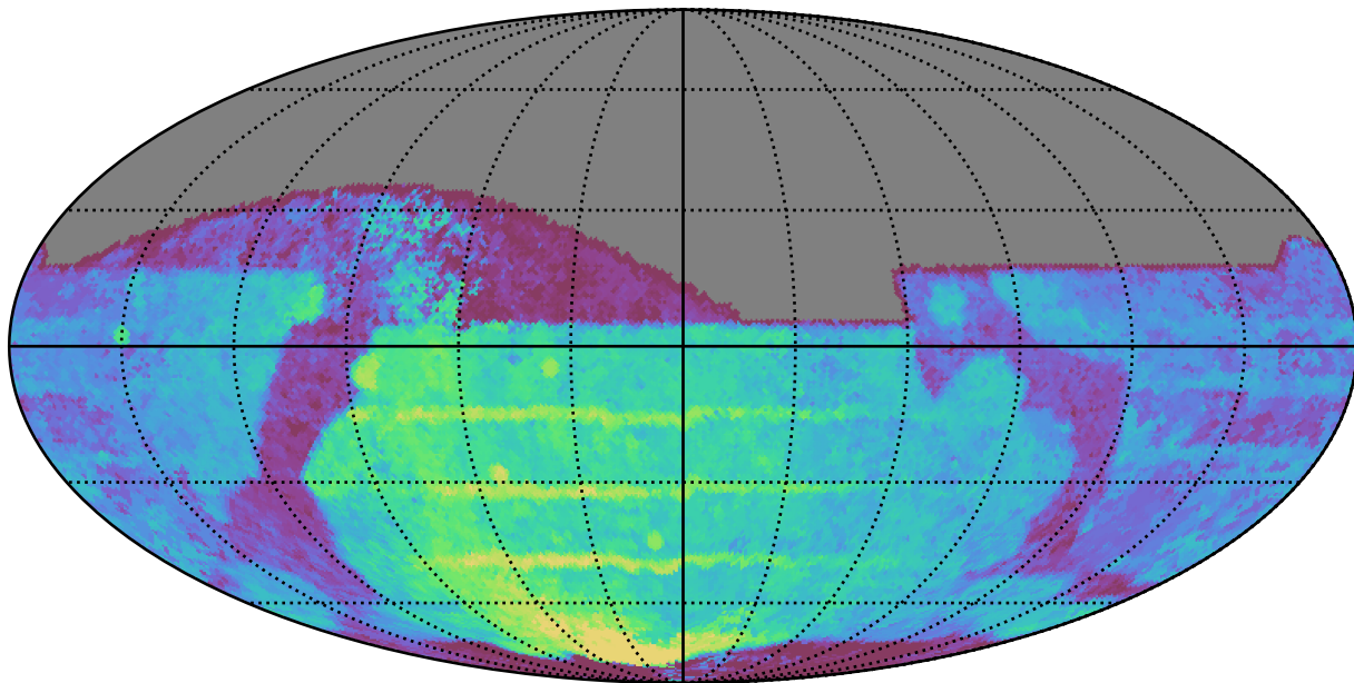
weather_cloudso12v3.4_10yrs All sky z band: Median Season Length
