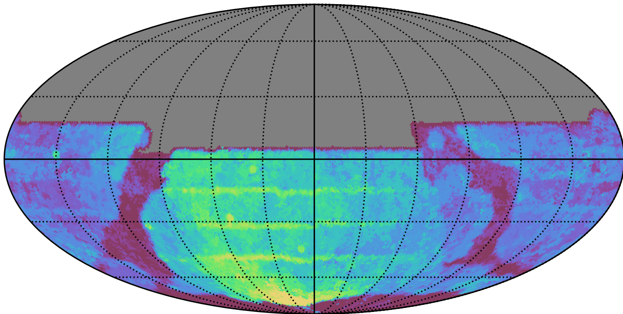
weather_cloudso12v3.4_10yrs All sky y band: Median Season Length
