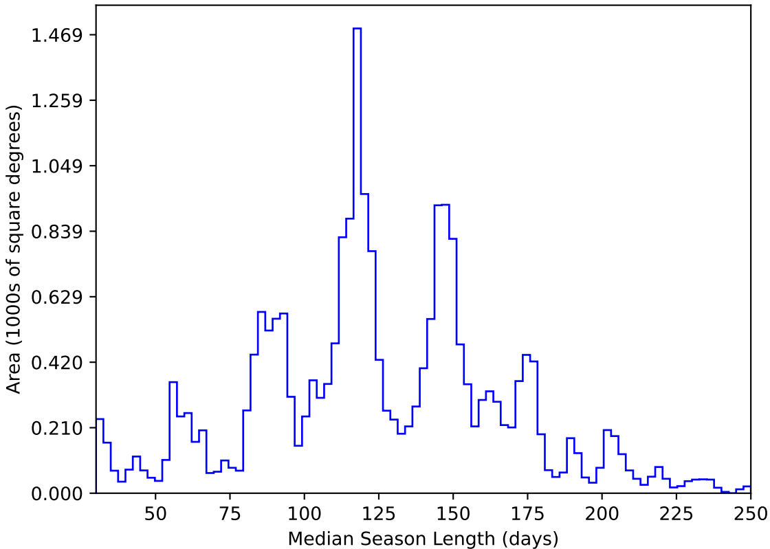
weather_cloudso12v3.4_10yrs All sky y band: Median Season Length
