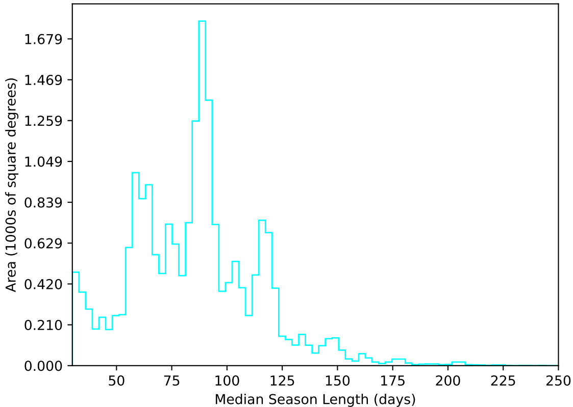
weather_cloudso12v3.4_10yrs All sky u band: Median Season Length
