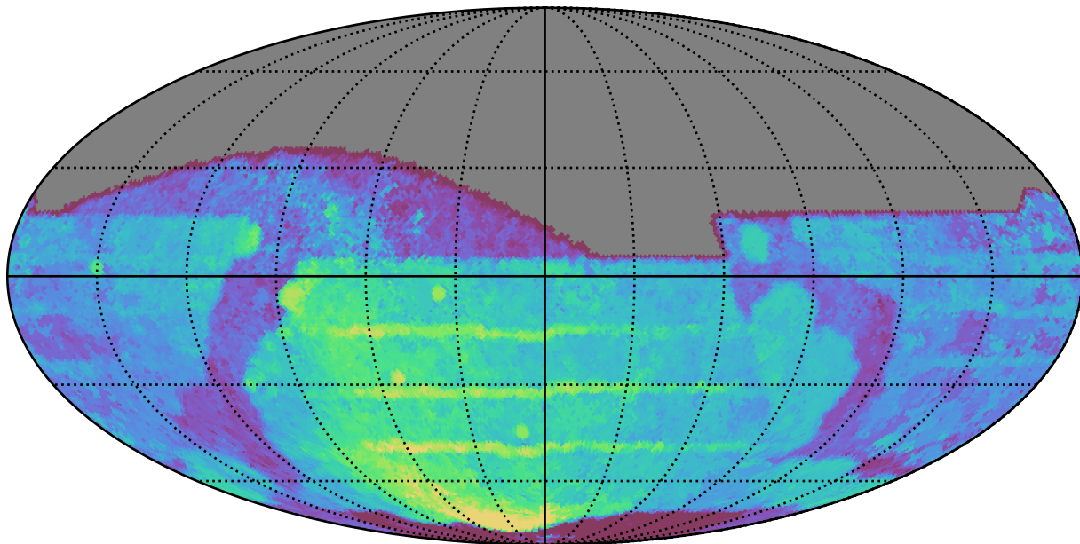
weather_cloudso12v3.4_10yrs All sky r band: Median Season Length
