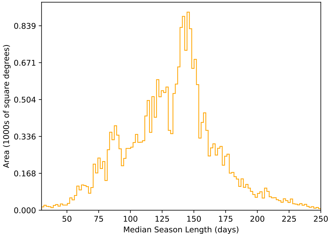
weather_cloudso12v3.4_10yrs All sky r band: Median Season Length
