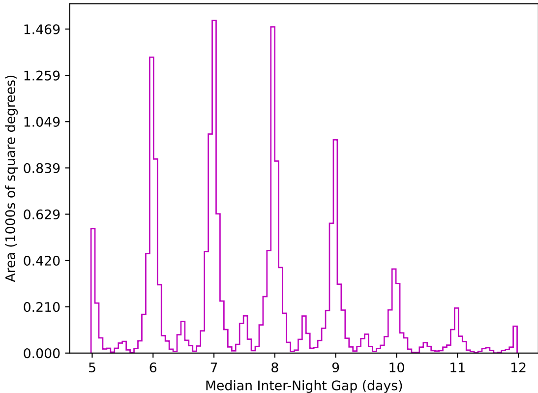
weather_cloudso12v3.4_10yrs WFD z band: Median Inter-Night Gap
