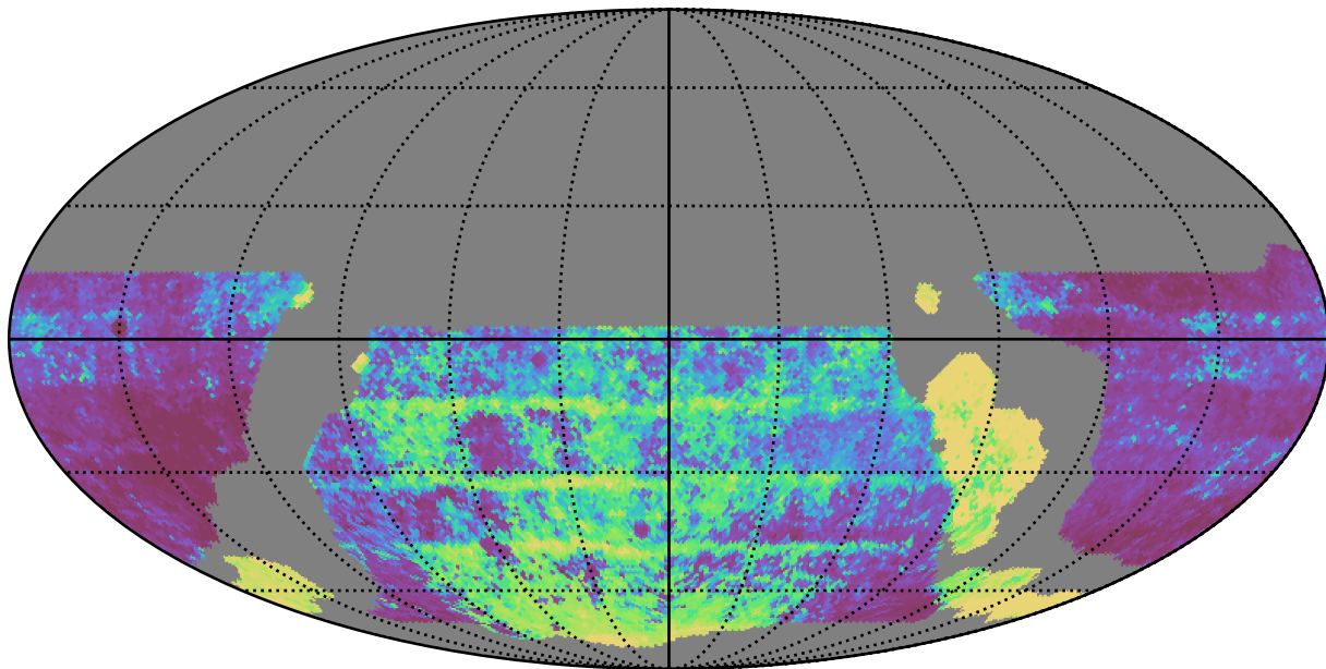
weather_cloudso12v3.4_10yrs WFD y band: Median Inter-Night Gap
