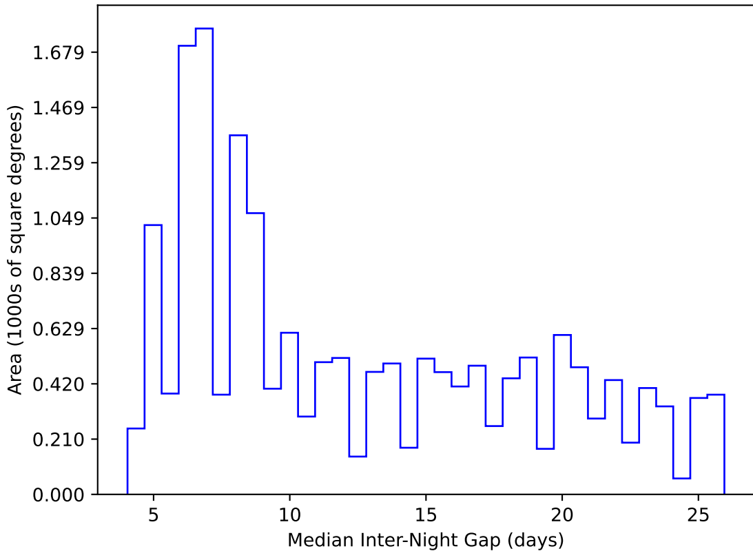
weather_cloudso12v3.4_10yrs WFD y band: Median Inter-Night Gap
