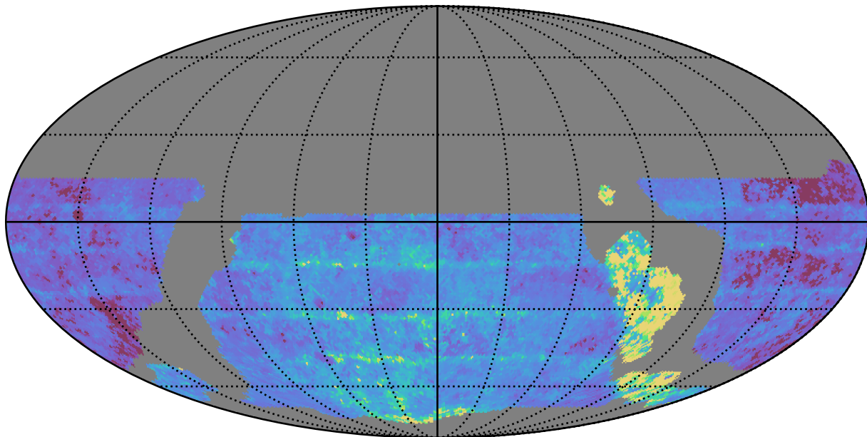
weather_cloudso12v3.4_10yrs WFD u band: Median Inter-Night Gap
