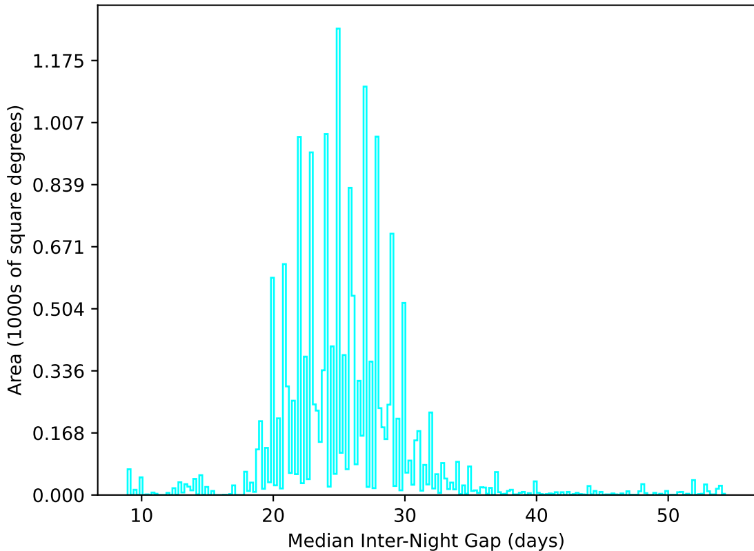
weather_cloudso12v3.4_10yrs WFD u band: Median Inter-Night Gap
