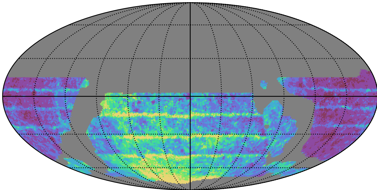
weather_cloudso12v3.4_10yrs WFD r band: Median Inter-Night Gap
