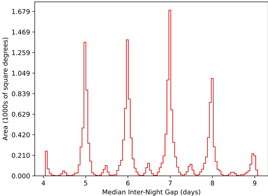
weather_cloudso12v3.4_10yrs WFD i band: Median Inter-Night Gap
