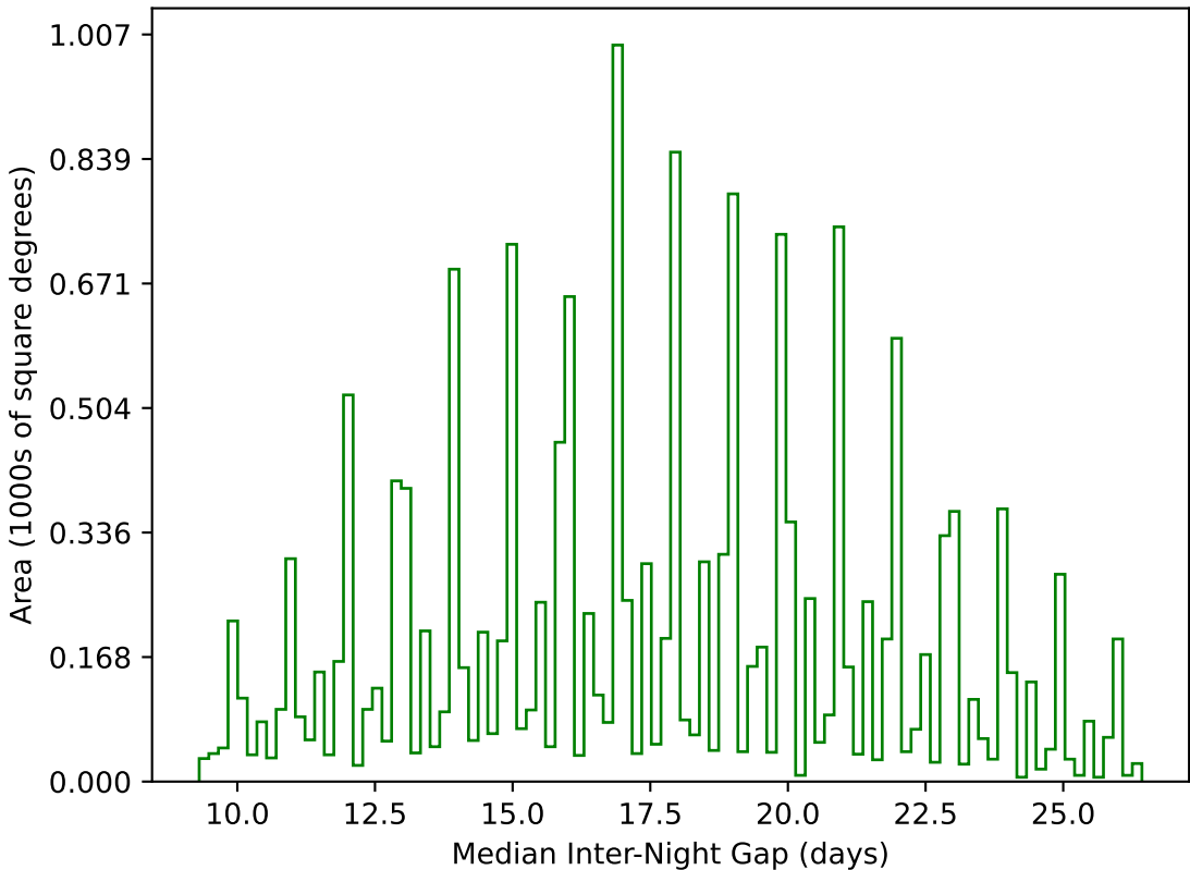
weather_cloudso12v3.4_10yrs WFD g band: Median Inter-Night Gap
