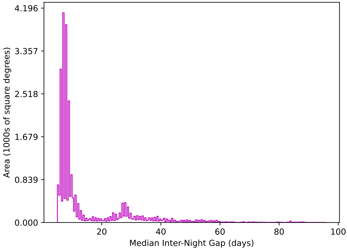
weather_cloudso12v3.4_10yrs All sky z band: Median Inter-Night Gap
